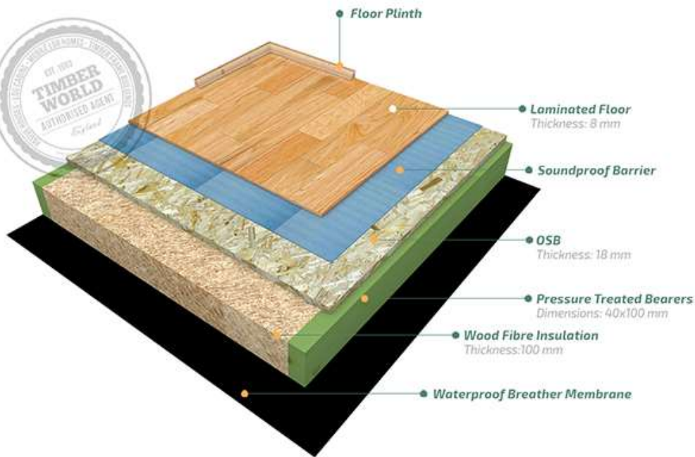
Laminated Floor Structure
